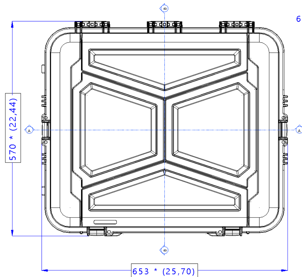
Vista Coperchio Lid View
