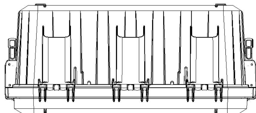
Vista Coperchio Lid View
