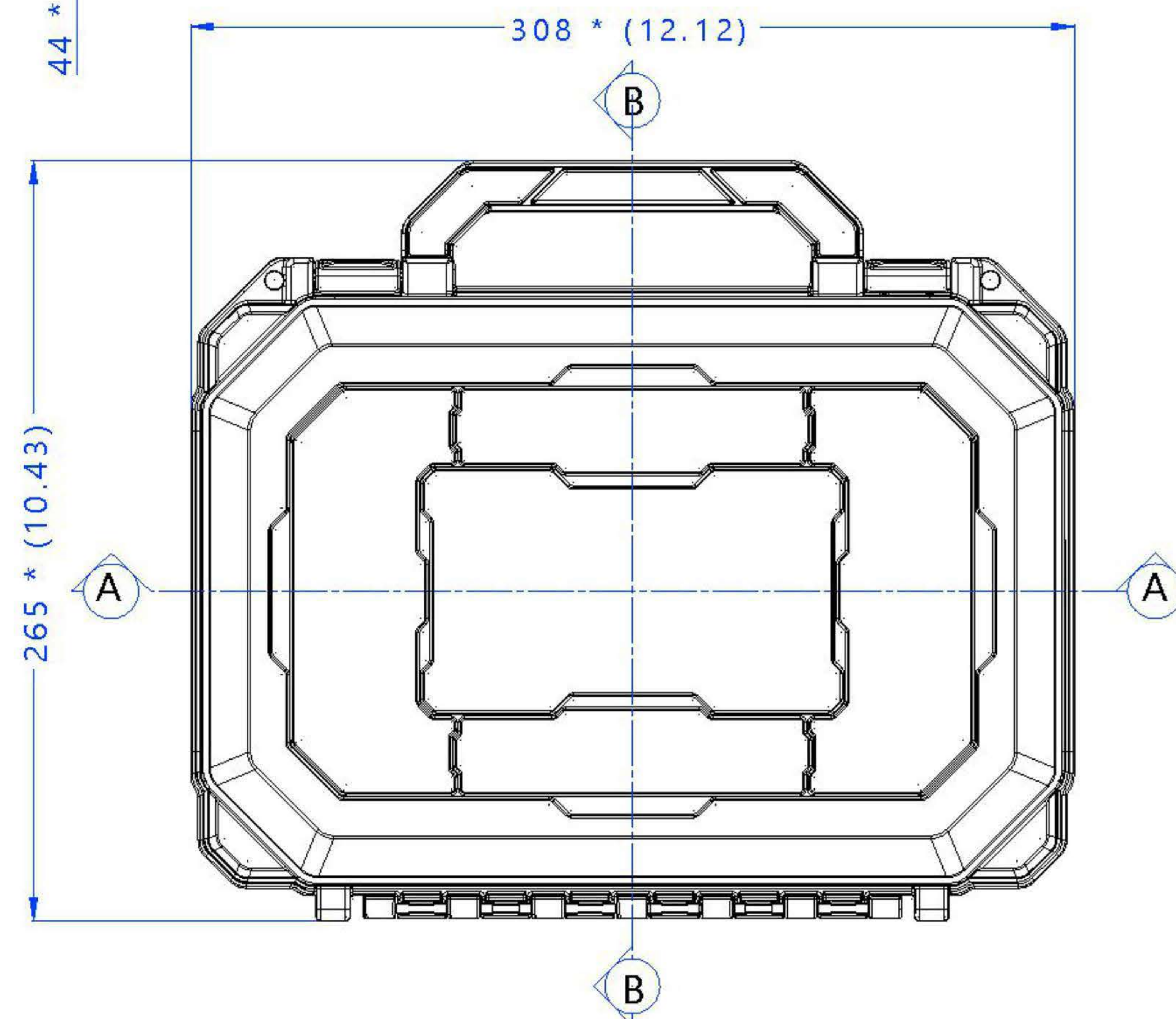
Vista Coperchio Lid View
