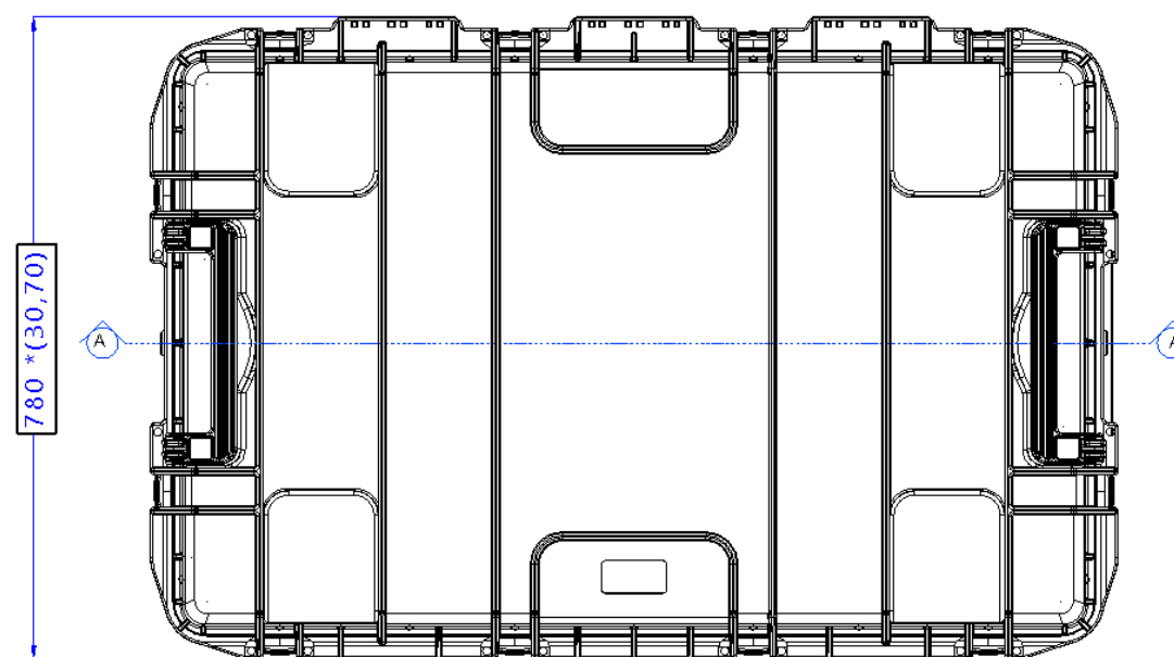
Vista frontale Front view
