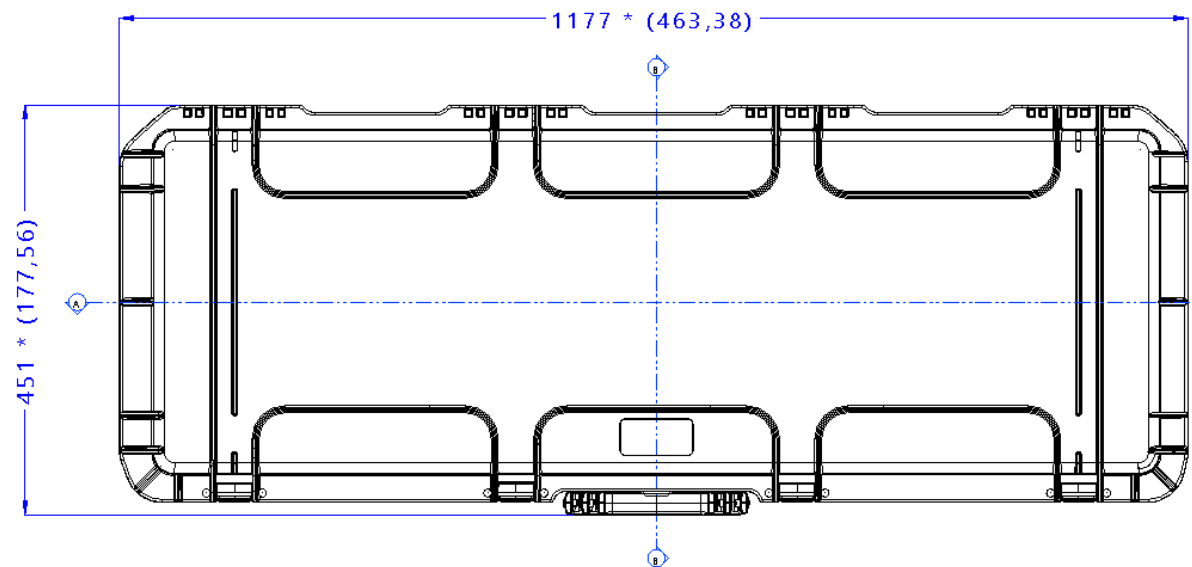
Vista Coperchio Lid View
