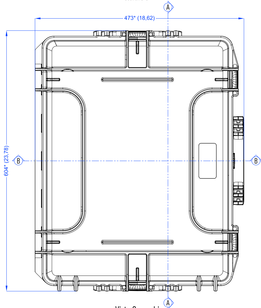
Vista Coperchio Lid View
