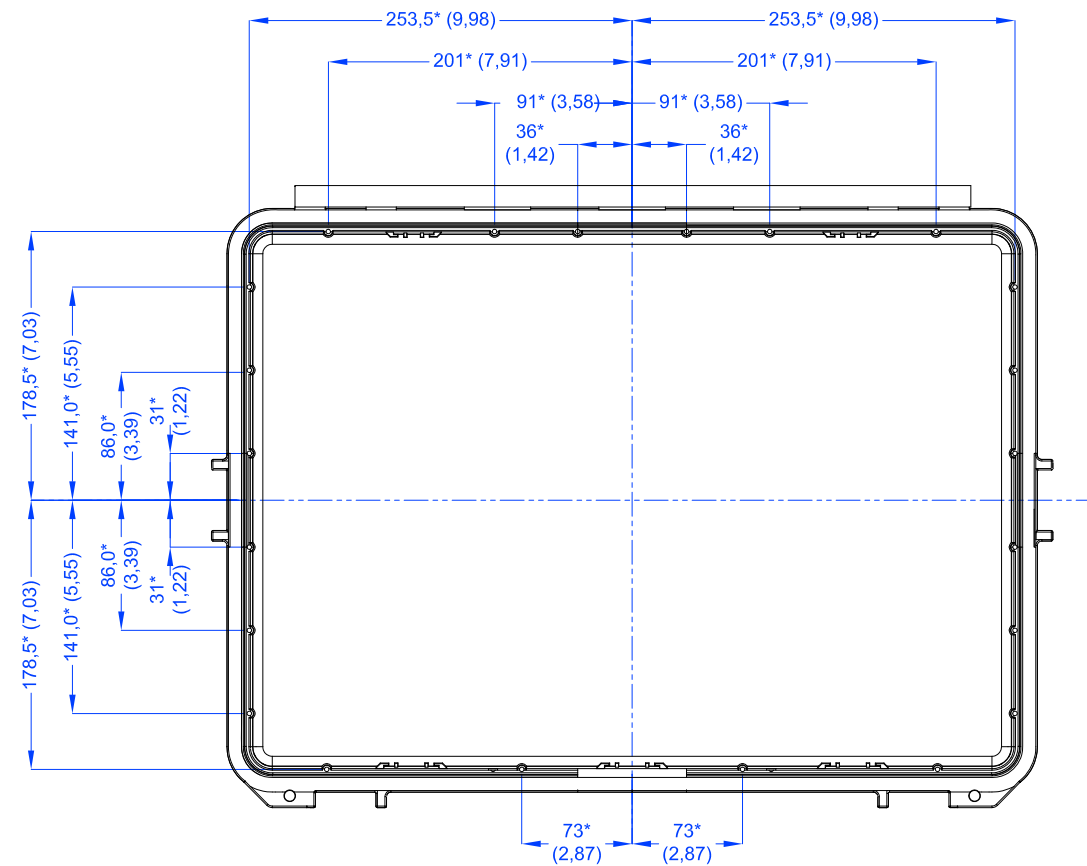
Vista Interna Coperchio Lid Inner View
