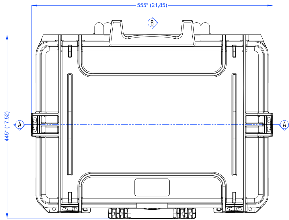
Vista Coperchio Lid View
