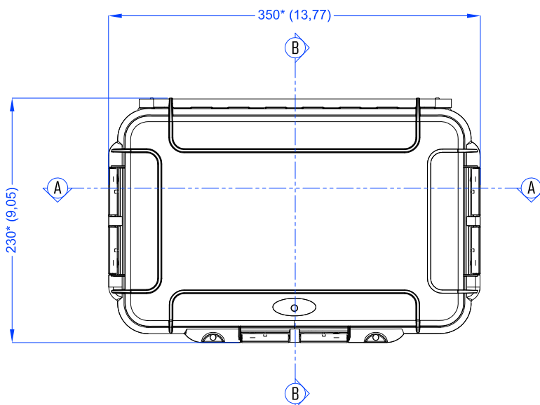
Vista Coperchio Lid View
